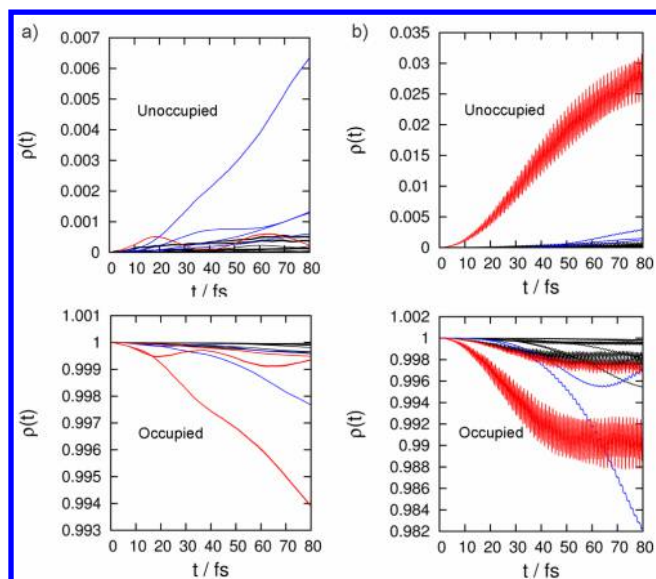
Figure 11. Occupied (bottom) and unoccupied (top) orbital population evolution for \text{Ti}_{17}\text{C343}_2 during electron injection at (a) 221 and (b) 424 nm.
