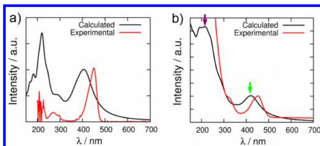
Figure 6. Simulated absorption spectrum for both free C343 (a) and \text{Ti}_{17}\text{C343}_2 (b). Magenta and green arrows indicate the wavelengths at which electron and hole injection take place, respectively.
