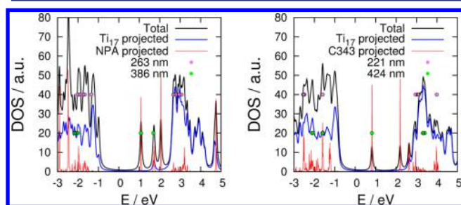
Figure 12. Left: DOS for \text{Ti}_{17}\text{NPA}_4 . Dots indicate the states that participate the most in the excitation. Right: DOS for \text{Ti}_{17}\text{C343}_2 . Very narrow Lorentzian functions of \text{fwhm} = 0.01 eV were employed for the projections onto the dyes, while 0.1 eV was used for the total and \text{Ti}_{17} projected DOS. The plots were shifted such that E_F = 0.0 eV.
