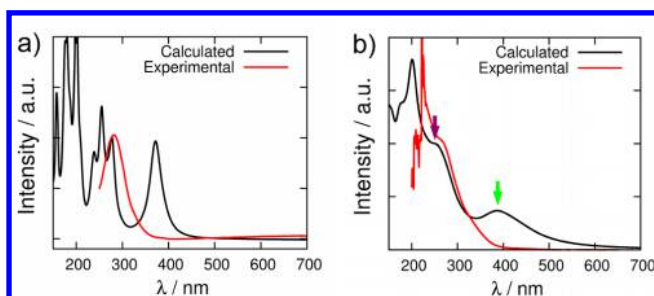
Figure 8. Simulated absorption spectrum for both free NPA (a) and \text{Ti}_{17}\text{NPA}_4 (b). Magenta and green arrows indicates the wavelengths at which electron and hole injection take place, respectively.
