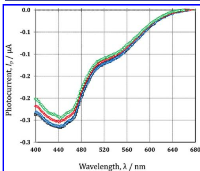
Figure 15. Negative (cathodic) photocurrent recorded for \text{Ti}_{17}\text{NPA}_4 supported by a FTO working electrode. Four successive measurements are shown.
