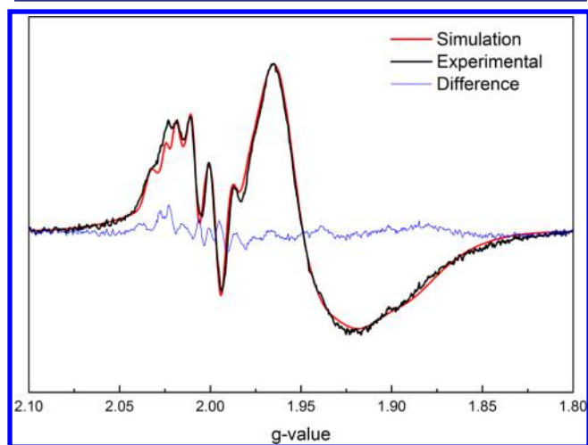
Figure 3. Light-minus-dark EPR spectra of unfunctionalized \text{Ti}_{17} 5 in frozen dichloromethane solution at 7 K illuminated at \lambda > 295 nm. The sum of the simulated basis spectra (red) is compared to the experimental spectrum (black). The difference between the experimental and simulated spectra is shown in blue.
