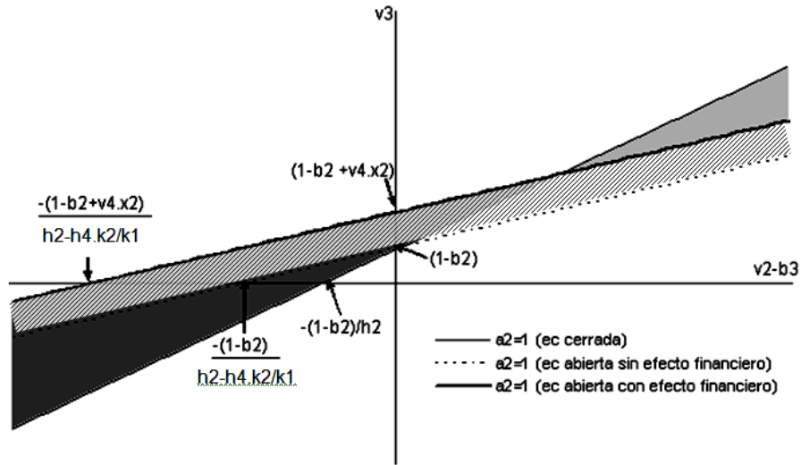
(a) h_2 > h_4.k_2/k_1
