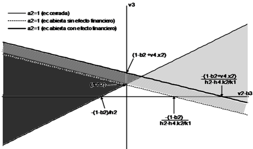
(b) h_2 < h_4.k_2/k_1
