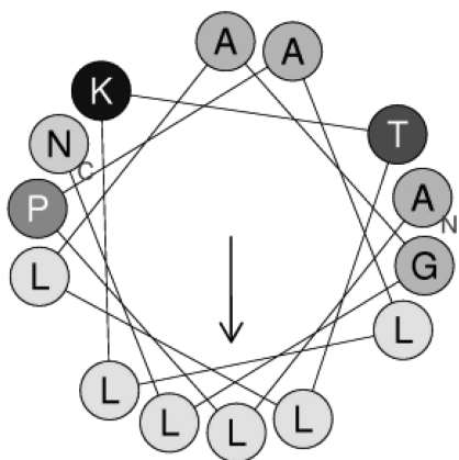
Figure 3. Schiffer–Edmundson wheel projection of P3-Hp-1891. The representation was done using Heliquest software ( http://heliquest.ipmc.cnrs.fr/ ). The window of analyses was limited to the helical region (5–18), determined on the basis of the data obtained by PSIPRED and GOR V. Amphipathic moment ( \mu ): 0.533.
