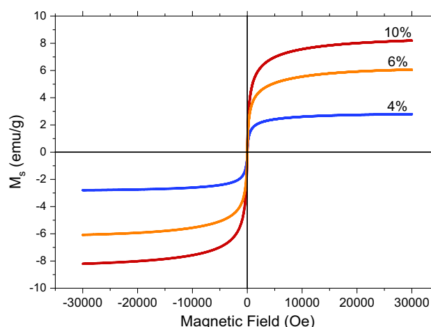
Fig. 3 Magnetic hysteresis loop for MPVA
