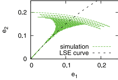
Figure 12. Comparison between the computation of the LSE curve and the result of numerical simulation for the CoRoT-7 system (without the contribution of the relativistic potential). After the angle \Delta\varpi is close to 0^\circ (Mode I), both curves are almost coincident.
