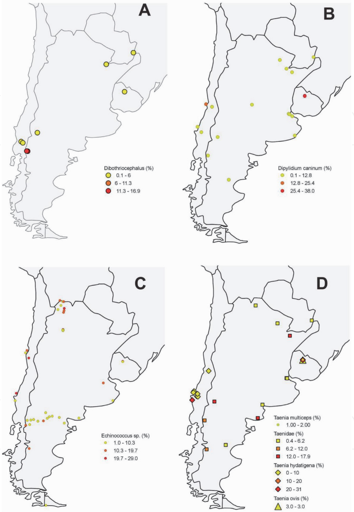
Figure 3. Distribution of Cestoda collected in Argentina, Chile and Uruguay. A.: Dibothriocephalus sp.; B.: Dipylidium caninum; C.: Echinococcus sp.; D.: Taenids .
