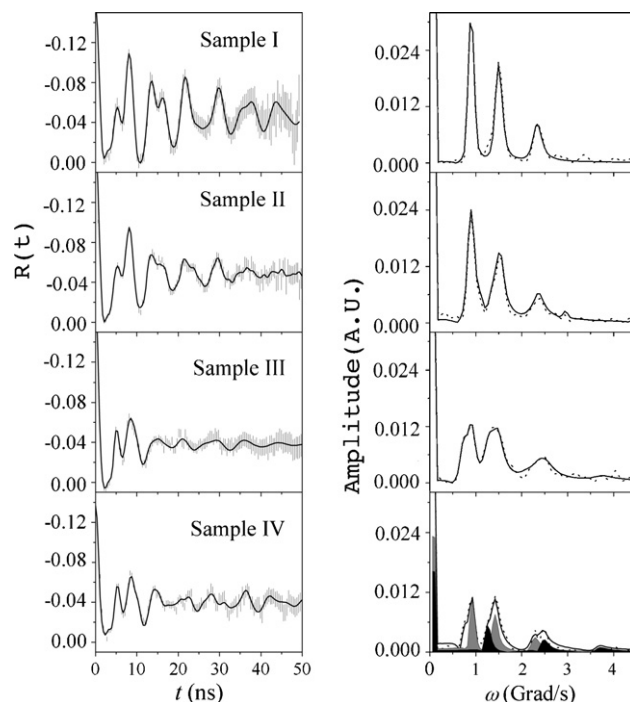
Fig. 2. R(t) spectra (left) and their corresponding Fourier transforms (right) of (^{181}\text{Hf} \rightarrow ^{181}\text{Ta}) in the \text{Tm}_2\text{O}_3 sample series (see Section 2.2 and Table 1) taken at RT in air. The frequencies \omega_n associated with the hyperfine interactions Hfi 2 and Hfi 3 are shaded in grey and black, respectively, in the fourth Fourier spectrum. Note the change in scale of this spectrum.
