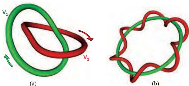
Fig. 2. Linked flux tubes.
