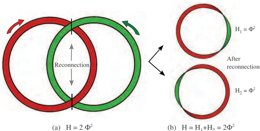
Fig. 4. (a) Two linked ribbon-like flux tubes undergo a localized reconnection process that give rise to two separate but twisted tubes (b). The global helicity of the system is conserved.
