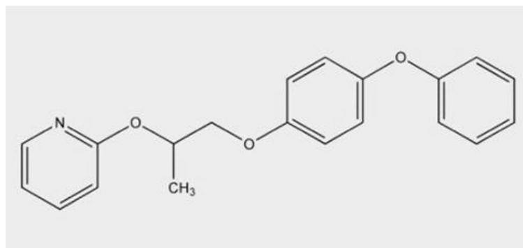
Fig. I.3. Chemical structure of pyriproxyfen
