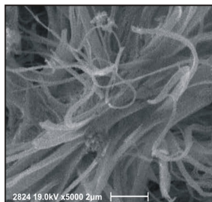
Fig. 6. Bundles of nanotubes and nanobelts (SEM).
