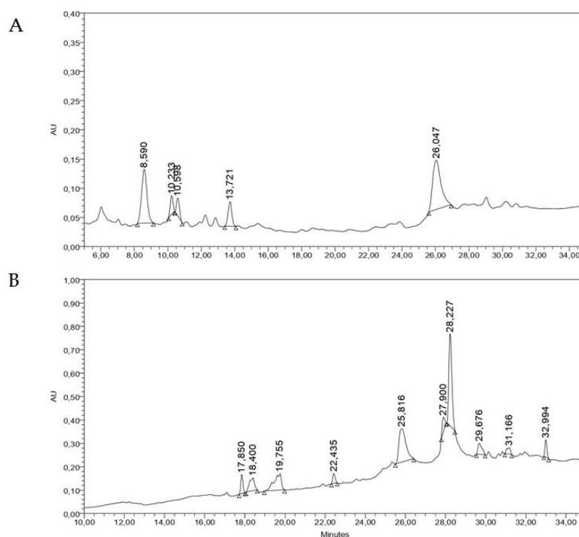
Figure 5. HPLC analysis of (A) MGPU and (B) MCM. (Chromatographic system: stationary phase: C-18; mobile phase: 15–85% MEOH in 35 min; detector: PDA, 210 nm).
