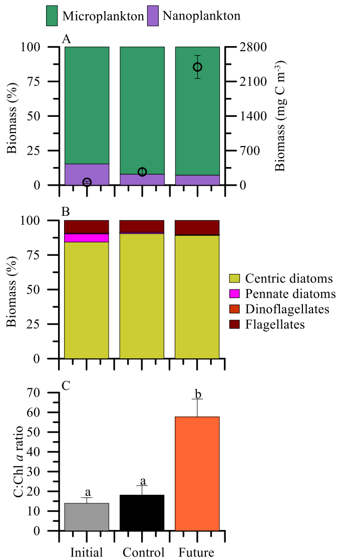
Fig. 2. Mean ( \pm SD) contribution of micro- and nanophytoplankton to total carbon biomass (%) and total biomass (concentration, black circles) (A), contribution of the different taxonomic groups (B), and total carbon to chlorophyll a ratio (C) at the initial and at the end of the experimental period in plankton communities exposed to Control and Future environmental conditions. Letters on top of the bars represent significant differences by the Least Significant Differences post hoc test.
