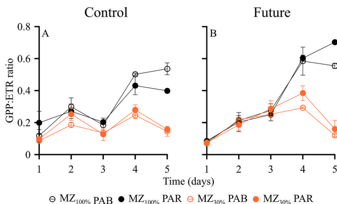
Fig. 5. Mean ( \pm SD) ratio of gross primary production (GPP; in \mu\text{mol O}_2 \mu\text{g Chl a}^{-1} \text{h}^{-1} ) to electron transport rates (ETR; in \mu\text{mol e}^- \mu\text{g Chl a}^{-1} \text{h}^{-1} ) in plankton communities exposed to Control (A) and Future (B) environmental conditions under full spectrum of solar radiation (PAB) versus only photosynthetically active radiation (PAR), and in presence (MZ 100% ) or absence (MZ 30% ) of microzooplankton over the experimental period. Higher GPP:ETR ratios indicate a lower photosynthetic efficiency, and vice versa.
