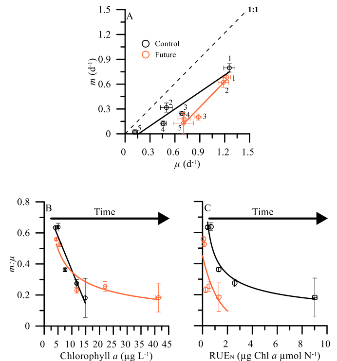
Fig. 6. Relationship between intrinsic phytoplankton growth ( \mu , in \text{d}^{-1} ) and microzooplankton grazing ( m , in \text{d}^{-1} ) rates (A), microzooplankton grazing pressure ( m:\mu ratio) vs. chlorophyll a (in \mu\text{g L}^{-1} ) (B), and vs. resource use efficiency of nitrogen ( RUE_N , in \mu\text{g Chl a} \mu\text{mol N}^{-1} ) (C) in plankton communities exposed to Control and Future environmental conditions over the experimental period. The dashed line represents the 1:1 m and \mu relationship, the black and orange solid lines represent linear or non-linear fittings, and numbers close to the symbols represent the experimental day. (For interpretation of the references to colour in this figure legend, the reader is referred to the Web version of this article.)
