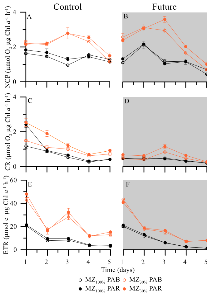
Fig. 4. Mean ( \pm SD) net community production (A, B) (in \mu\text{mol O}_2 \mu\text{g Chl a}^{-1} \text{h}^{-1} ), community respiration (C, D) (in \mu\text{mol O}_2 \mu\text{g Chl a}^{-1} \text{h}^{-1} ), and electron transport (E, F) (in \mu\text{mol e}^- \mu\text{g Chl a}^{-1} \text{h}^{-1} ) rates in plankton communities exposed to Control and Future environmental conditions under full spectrum of solar radiation (PAB) versus only photosynthetically active radiation (PAR), and in presence (MZ 100% ) or absence (MZ 30% ) of microzooplankton over the experimental period.
