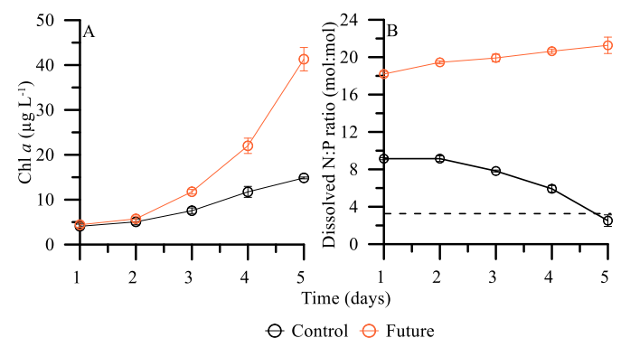
Fig. 3. Mean ( \pm SD) chlorophyll a (Chl a ) concentrations (A) and dissolved nitrogen to phosphorus ratios (N:P) (B) in plankton communities exposed to Control and Future environmental conditions over the experimental period. Dash line in panel B represents the N:P ratio at the sampling condition.
