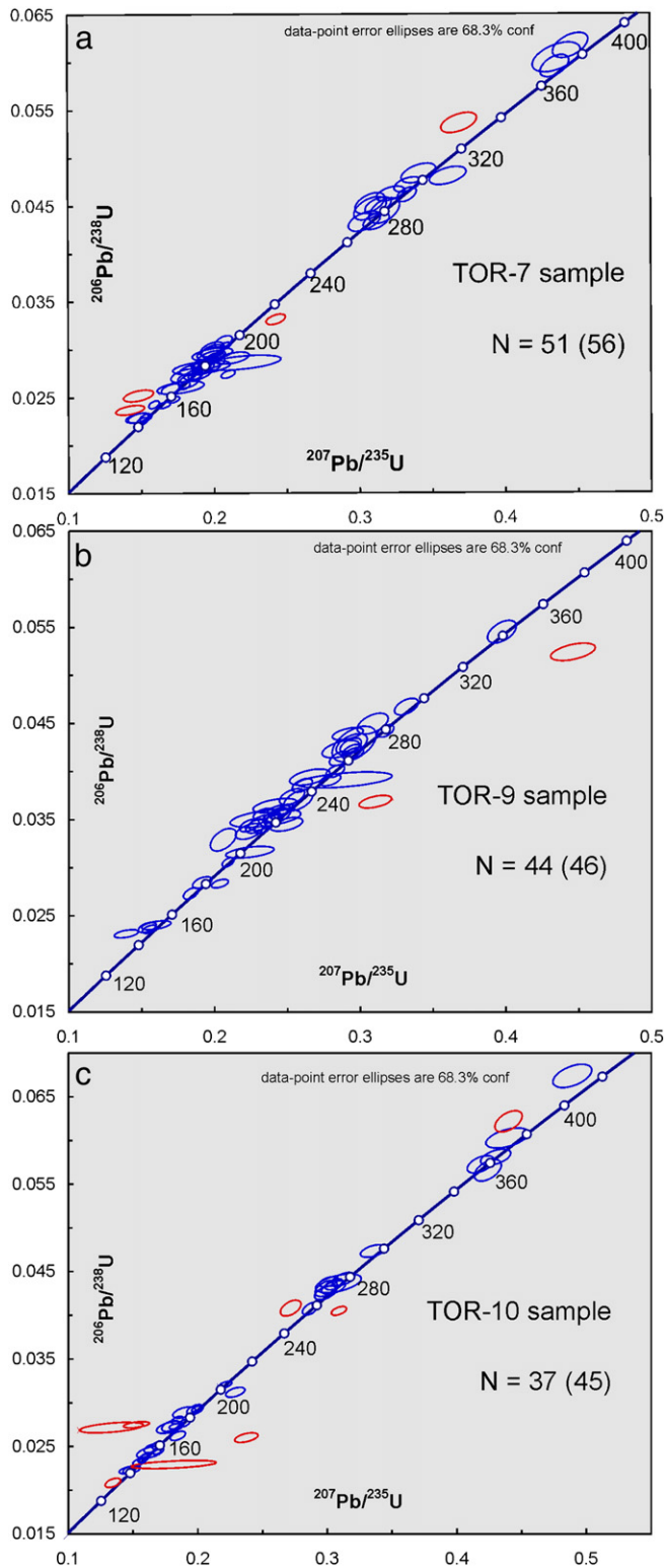
Fig. 10. Concordia plots from the U/Pb samples analyzed, a) TOR-07, b) TOR-09, and c) TOR-10. The detrital zircon ages shown in the concordia plots are the concordant ages (in blue) and discordant ages (in red) discussing in the text. One discordant age falls outside of the TOR-07 diagram (a).
