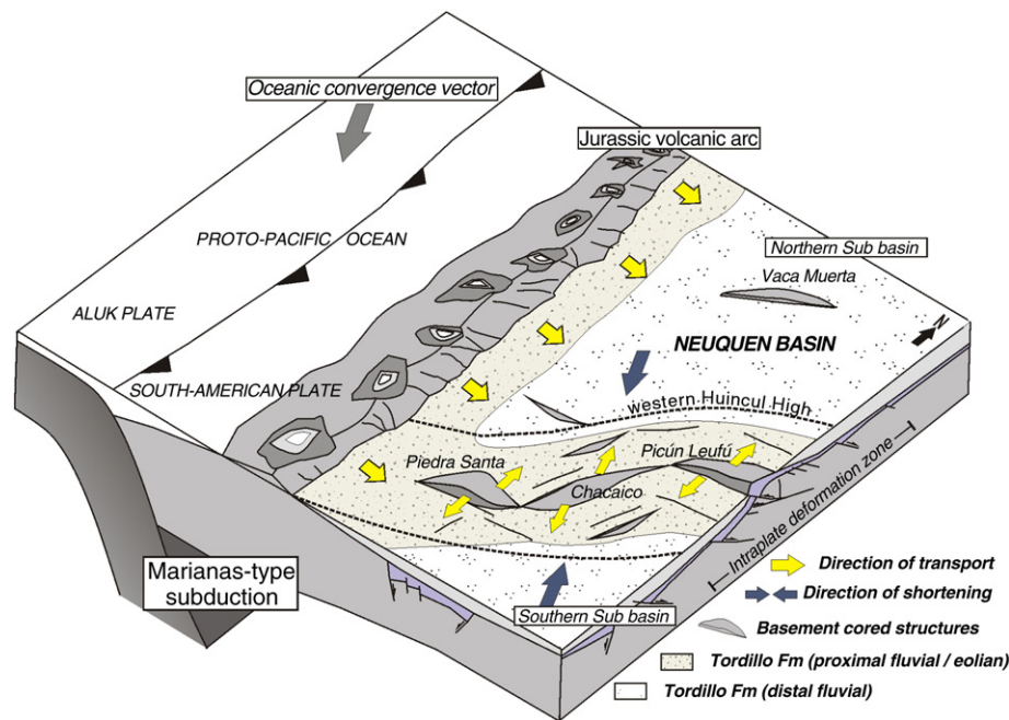
Fig. 13. Late Jurassic paleogeography and geological setting of the Neuquén Basin. Note the potential source areas for the basin: presence of a western magmatic arc and emerged areas along the east–west oriented Huincul deformational zone.
