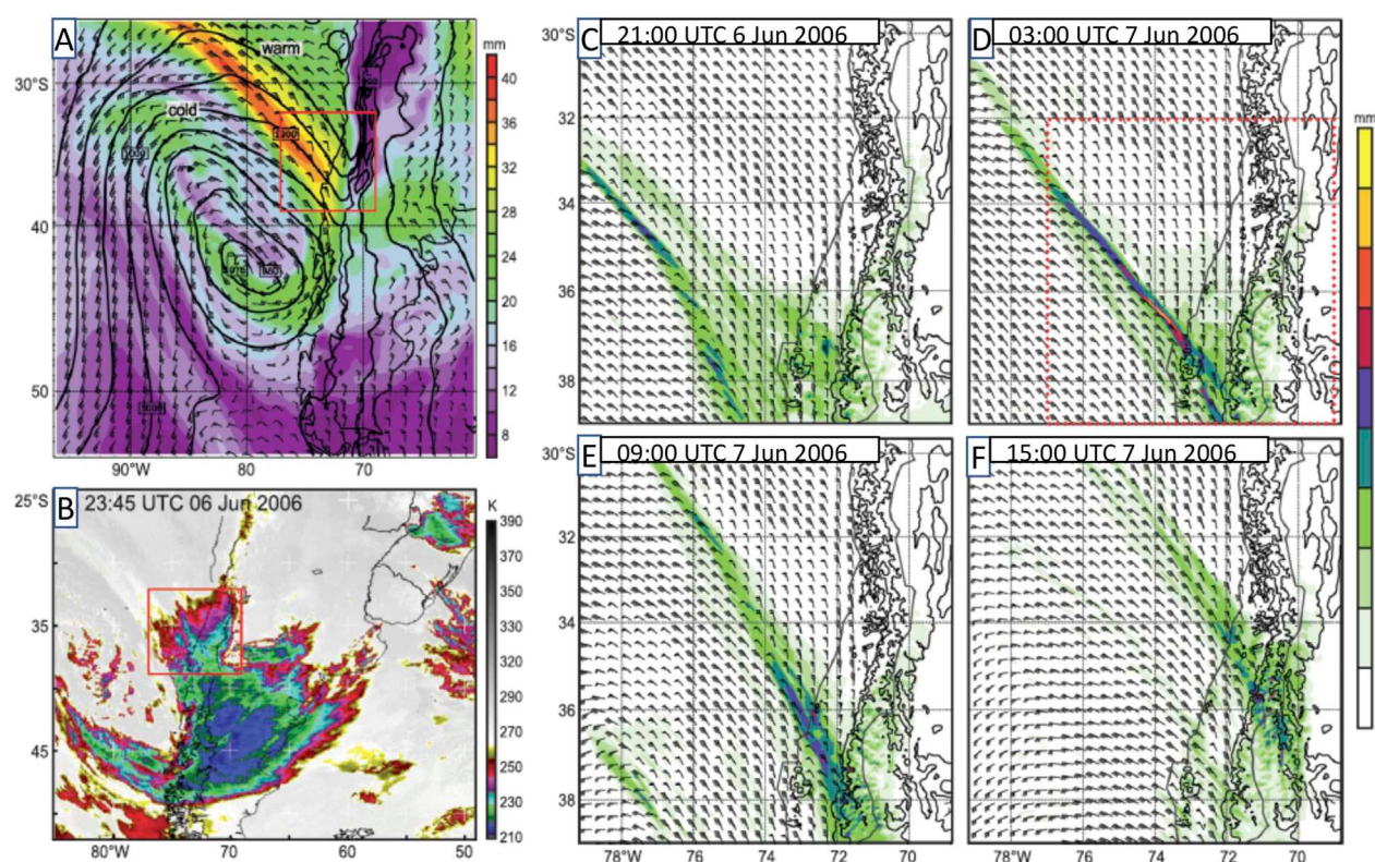
FIGURE 4 Blocking and other orographic processes associated with a cold-frontal rainband in the subtropical Andes, from (A) 36-km WRF run at 00:00 UTC 7 June 2006, (B) Infrared satellite data, (C–F) 3-km WRF run. (A) Surface pressure (black contours, every 5 hPa), 925 hPa windbarbs and precipitable water (shaded). (C–F) Wind barbs at 0.5 km and 1-h accumulated precipitation (shaded; mm). Full barb = 5 m s -1 . Solid black lines are 500 m and 1,000 m terrain altitudes. Source: Viale et al. (2013) . © American Meteorological Society. Used with permission.
