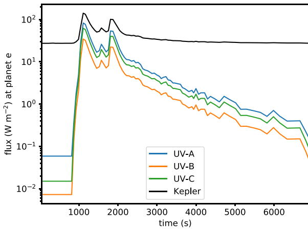
Figure 2. Observed flare light curve in the Kepler band (black) in comparison with the modelled UV-A (blue), UV-B (orange), and UV-C (green) curves. The fluxes are scaled to the orbit of planet e , and a flare temperature of 9000 K was assumed.
