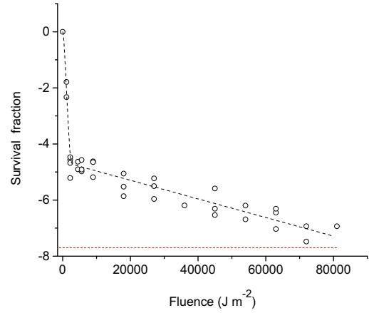
Figure 5. Survival curve obtained for D. radiodurans at different fluences of germicidal radiation. The survival fraction is the \log(N/N_0) . The black line corresponds to a fit obtained with a kinetic model and the red line corresponds to the LOD.
