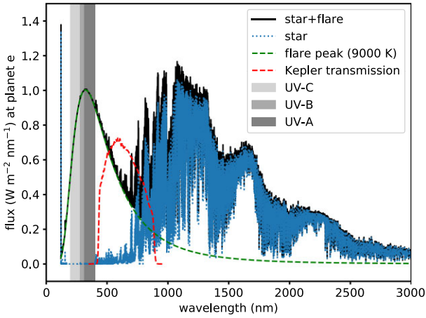
Figure 1. Quiescent stellar spectrum (blue), superflare peak spectrum (green; blackbody with 9000 K), and total spectrum (black) scaled to the orbit of TRAPPIST-1 e . The Kepler transmission curve is shown in red, and the relevant UV ranges as grey shaded areas.
