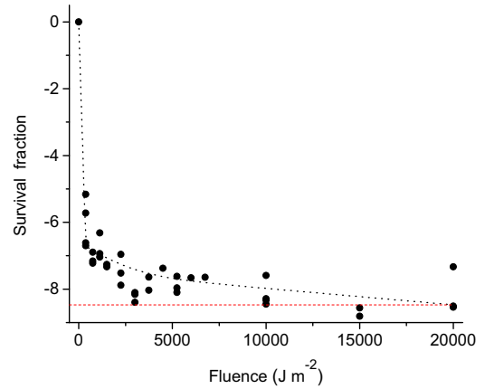
Figure 6. Survival curve obtained for E. coli at different fluences of germicidal radiation. The survival fraction is the \log(N/N_0) . The black line corresponds to a fit obtained with a kinetic model and the red line corresponds to the LOD.
