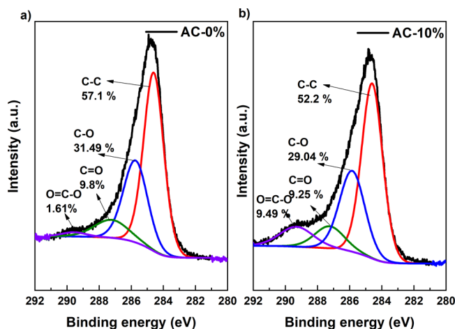
Figure 3. XPS deconvoluted spectra for C 1s of the (a) AC-0% and (b) AC-10% samples.
