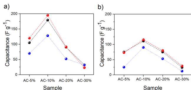
Figure 6. Specific capacitance of the different purple-corn-cob-based AC samples measured by different techniques: CV at 5 mVs -1 (black circles), GCD at 0.5 A g -1 (red circles), and EIS (blue circles) using (a) 1 mol L -1 H 2 SO 4 and (b) 1 mol L -1 KOH as electrolyte solutions.
