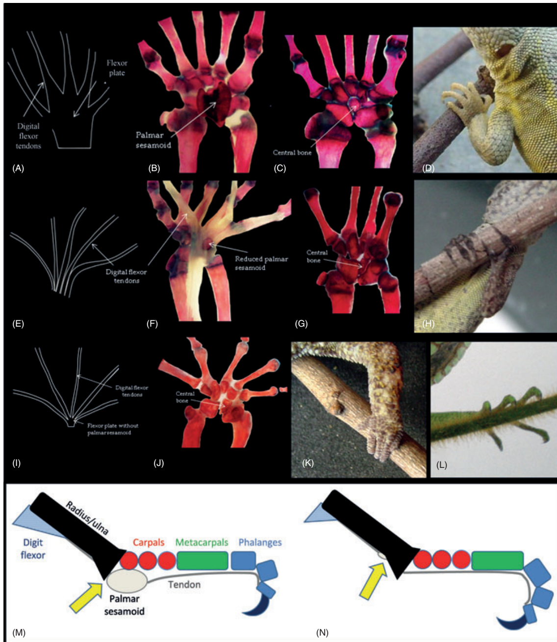
Fig. 3. (A–D) Liolaemus cuyanus right manus: (A) Schematic representation of the L-pattern (Moro & Abdala, 2004). (B) Ventral view showing the location of the palmar sesamoid. (C) Ventral view showing the carpal bones surrounding the central bone. (D) Dorsal view of L. crepuscularis left manus, showing partial digital flexion. (E–G) Anolis cristatellus right manus: (E) Schematic representation of a P-pattern (Moro & Abdala, 2004). (F) Ventral view showing the independence of the digital flexor tendons and the reduced palmar sesamoid. (G) Ventral view showing the shape and location of the central bone. (H) Ventral view of A. cristatellus right manus showing complete flexion of digits around branch. (I, J) Bogertia lutzae right manus: (I) Schematic representation of a G-pattern (Abdala et al. , 2009). (J) Ventral view showing the completely flat surface of the palm, and the shape and location of the central bone. (K) Dorsal view of Homonata fasciata left manus showing complete digital flexion around branch. (L) Left manus of Polychrus sp. showing opposition of digits I and V about its long (proximo-distal) axis, that presumably results from the position and shape of the central bone depicted in (G). (M, N) Schematic representation of proposed action of palmar sesamoids. (M) L-pattern tendon with large palmar sesamoid that becomes obstructed (yellow arrow) and limits excursion of m. flexor digitorum tendon, and results in flexion of only proximal and distal interphalangeal joints. (N) P- or G-pattern tendon with reduced (P-pattern; yellow arrow) or no (G-pattern) palmar sesamoid, which allows complete excursion of the tendon and results in flexion of interphalangeal and metacarpo-phalangeal joints. Photos in D and K by G. Scrocchi; H by J. Daza, and L by A. Herrel; all others by M.J. Tulli. Tendon schematics reprinted from Tulli et al. (2012) by permission of John Wiley & Sons, Inc.
