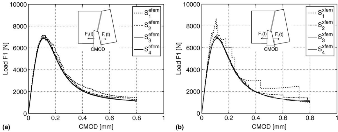
Fig. 6. 2D double-cantilever-beam (DCB) test with diagonal loads. Equilibrium curves (load F_1 vs. CMOD): (a) E-FEM and (b) X-FEM solutions.
