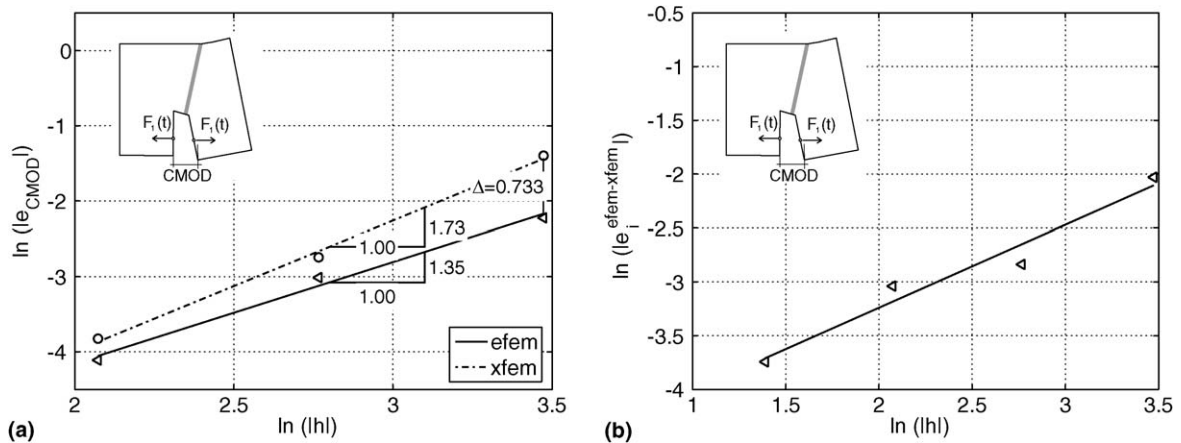
Fig. 8. 2D double-cantilever-beam (DCB) test with diagonal loads: (a) relative errors vs. element size and (b) E-FEM – X-FEM differences vs. element size h .
