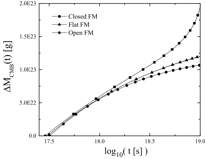
Fig. 1 Plots of the function \Delta M_{\text{BH}}^{\text{CMB}}(t) as a function of the cosmic time for the closed, flat, and open Friedmann models (FM)
