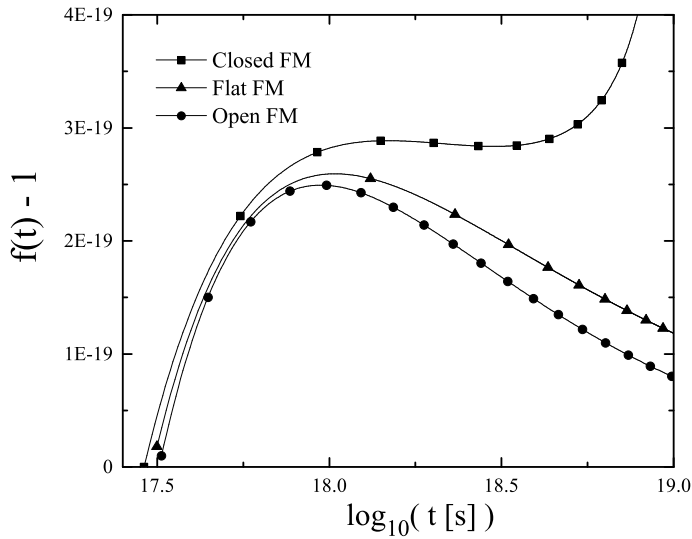
Fig. 2 Plots of the function f(t) - 1 as a function of the cosmic time for the closed, flat, and open Friedmann models (FM).
