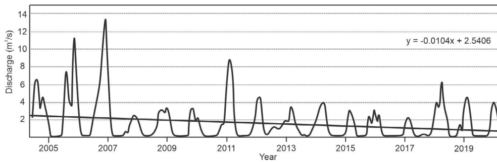
Fig. 6. Annual discharge of the Deseado River (m³/s) at Route 39 (interval 2004-2019).
