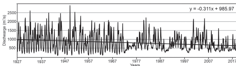
Fig. 3. Discharge (m 3 /s) of the Negro River at Primera Angostura (1927-2021). Floods were reduced since the dams' constructions during the seventies.
