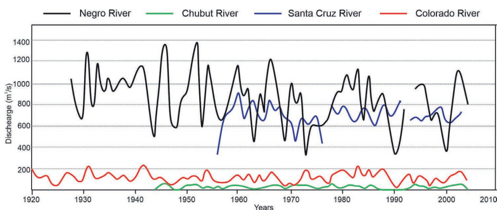
Fig. 2. Annual means of the rivers discharges. Negro (Primera Angostura station) and Santa Cruz (Charles Fuhr station) rivers have captured other watersheds while Colorado (Pichi Mahuida station) and Chubut (Los Altares station) watersheds were captured or became less operative.
