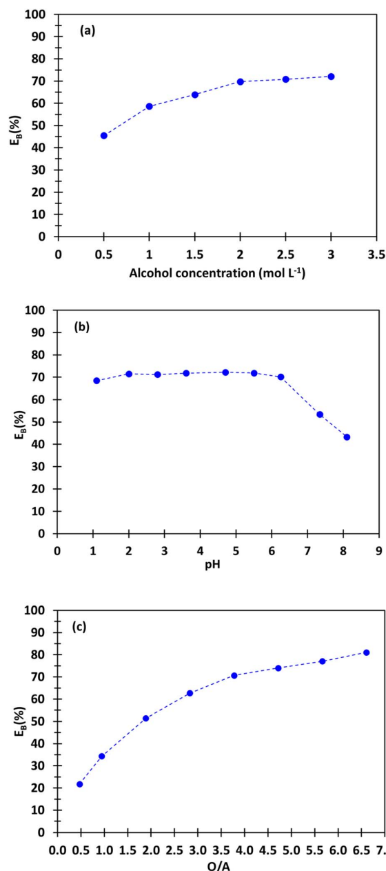
Fig. 3 Influence of (a) 2-butyl-1-octanol concentration in kerosene ( O/A = 4 , pH = 1 , 25 °C), (b) pH ( O/A = 4 , extraction solvent: 2 mol L^{-1} 2-butyl-1-octanol, 25 °C) and (c) O/A ( pH = 1 , extraction solvent: 2 mol L^{-1} 2-butyl-1-octanol in kerosene, 25 °C) on boron extraction efficiency from the synthetic brine (SB).
