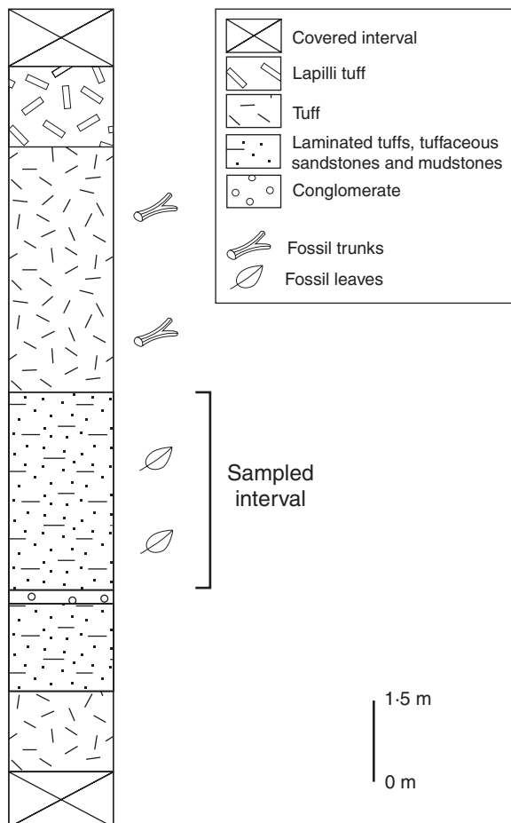
FIG. 2. Stratigraphic section of the Huitrera Formation at the Río Pichileufú flora site, showing the location of the fossil-bearing levels.
