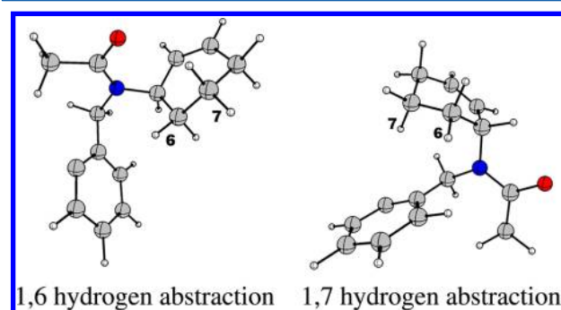
Figure 2. Conformers of radical 10 • suitable for hydrogen abstraction reaction.
