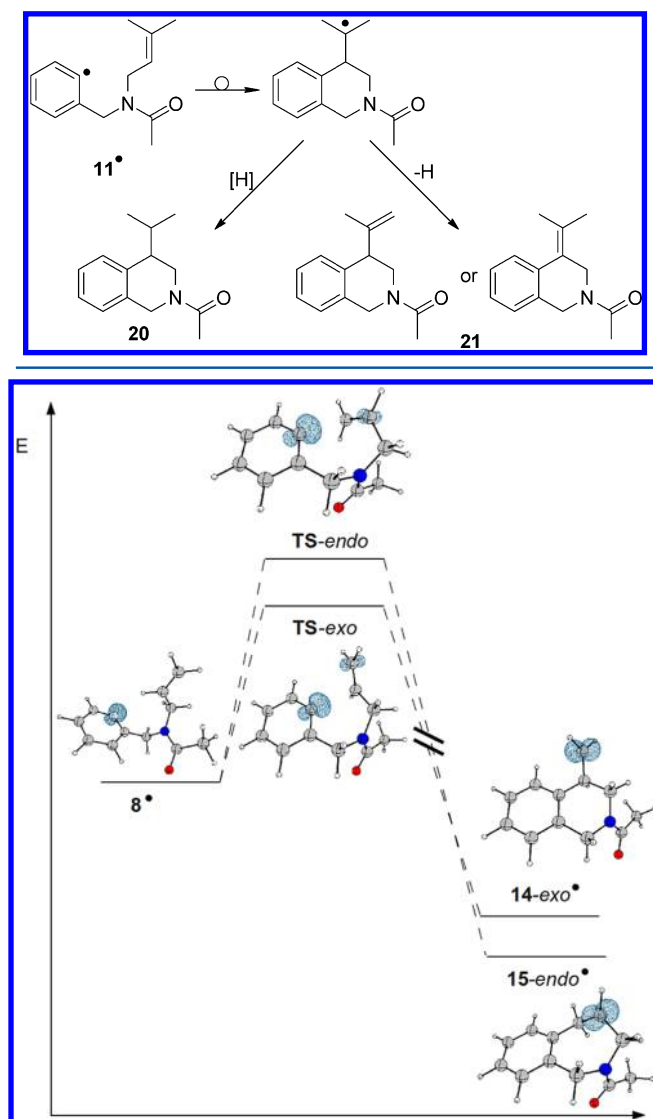
Figure 1. Schematic energy profile for the cyclization reaction. The aryl radical can cyclize in the exo or endo mode.
