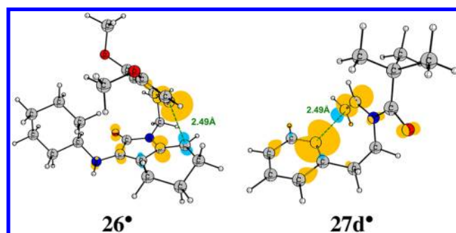
Figure 3. 7- endo cyclization TS. The spin density is delocalized over the \pi system.
