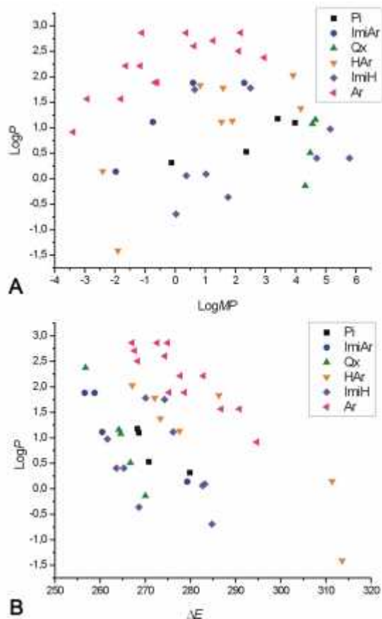
Figure 6. A. Correlations observed between hydrophobicity (LogP) and mutagenic potency (LogMP). B. Correlations between hydrophobicity (LogP) and nitrenium ion stability ( E_1 ).
