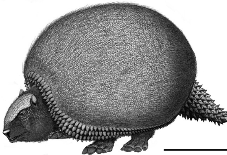
Fig. 4. Reconstruction of Glyptodon . Scale bar = 100 cm.
