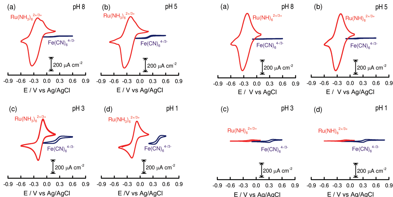
Figure 2. Cyclic voltammograms corresponding to a mesoporous silica film deposited on an ITO electrode in the presence of 1 mM Ru(NH 3 ) 6 3+ (red trace) and 1 mM Fe(CN) 6 3- , respectively, under different pH conditions: (a) 8, (b) 5, (c) 3, (d) 1.
