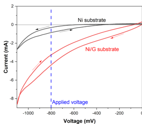
Figure 4. Cyclic Voltammograms corresponding to Ni (black) and Ni/G (red) electrodes.
