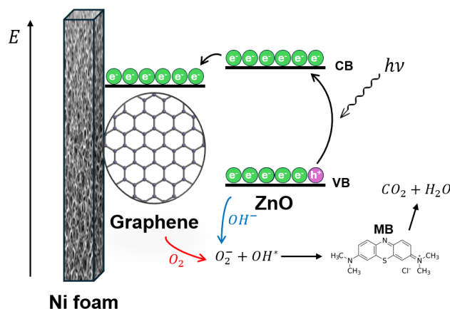
Figure 13. Scheme of the process with the ZnO and graphene bands.
