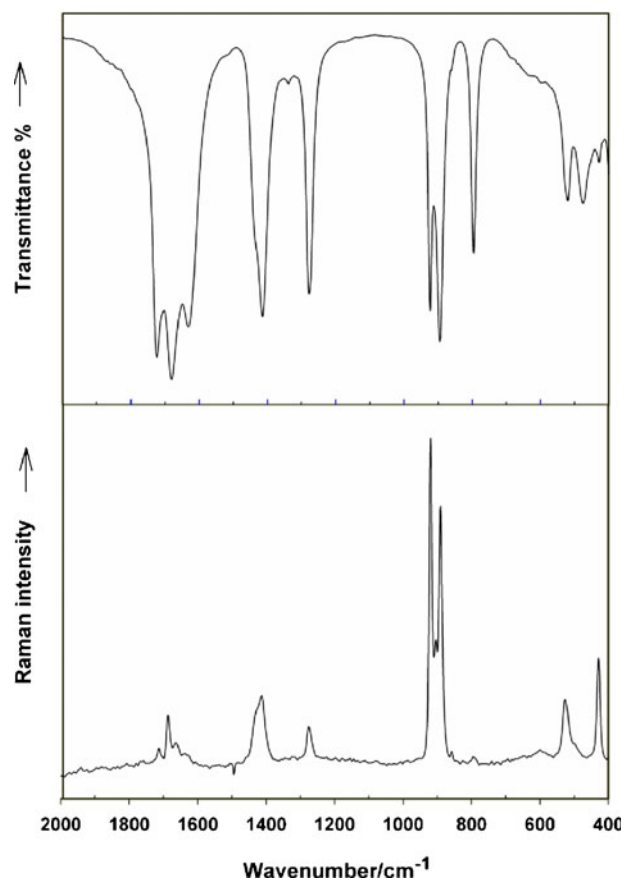
Fig. 2 FTIR ( above ) and FT-Raman ( below ) spectra of K_3[VO_2(C_2O_4)_2] \cdot 3H_2O in the spectral range between 2,000 and 400 cm^{-1}
