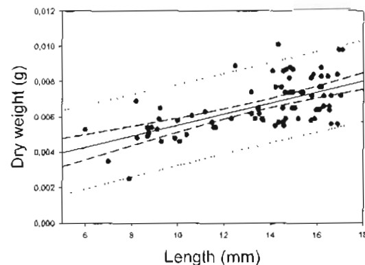
Figure 1. Linear regression of the length (mm) of E. timida with respect to its dry weight (g). Medium dash line corresponds to 95% confidence intervals; dotted line is the prediction intervals.
