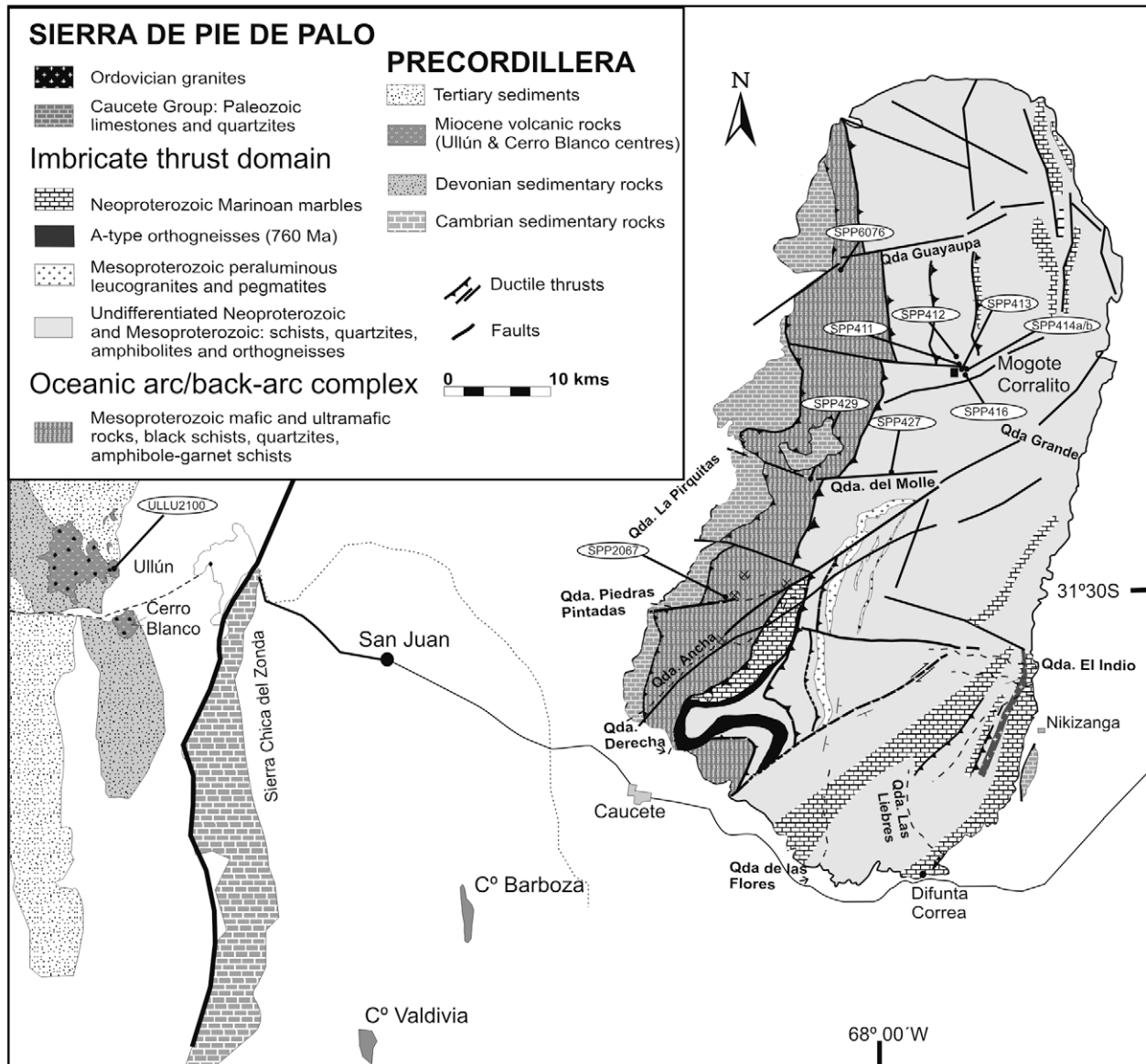
Fig. 3. Geological map of Sierra de Pie de Palo and adjacent Precordillera outcrops, modified after Vujovich and Kay (1998) and Baldo et al. (2006), with the location of samples considered in this work (Tables 3 and 4).
