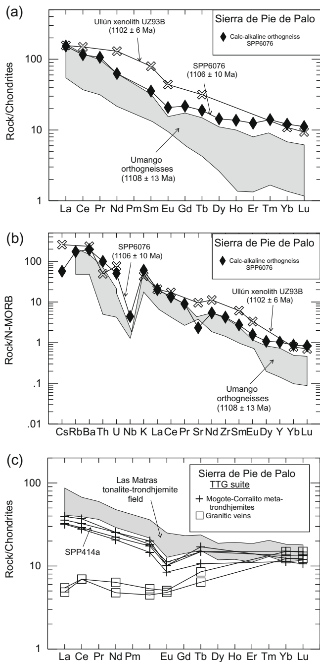
Fig. 10. (a) Trace element abundances in calc-alkaline meta-igneous rocks of Sierra de Pie de Palo normalized to chondrites (Nakamura, 1974) and (b) N-MORB (Sun and McDonough, 1989). The fields of Umango orthogneisses are from Varela et al. (2003) and the Ullún xenolith is from Kay et al. (1996). (c) Trace element abundances in meta-trondhjemites and related granitic veins from Sierra de Pie de Palo normalized to chondrites. The field for the 1244 \pm 42 Ma tonalite-trondhjemites from Las Matras block (Fig. 1) is from Sato et al. (2000). Identified samples are those with U–Pb SHRIMP ages determined in this study.
