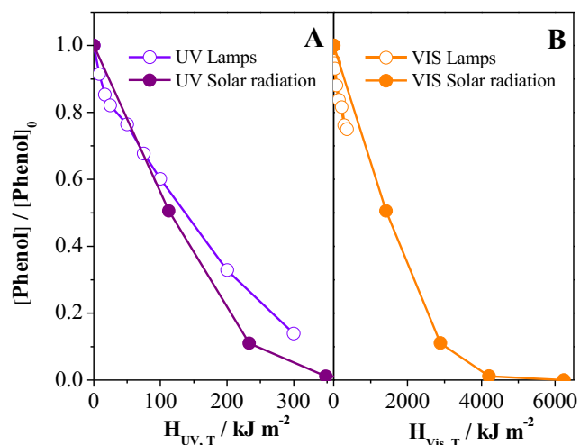
Fig. 5 Degradation of phenol 50 \mu\text{M} with 0.1Ce catalyst ( 1.0 \text{ g L}^{-1} ) as a function of the radiant exposure values: comparison between UV lamps and H_{\text{UV},T}^{\text{S}} after 3 h (A) and between VIS lamps and H_{\text{VIS},T}^{\text{S}} after 5 h (B)
