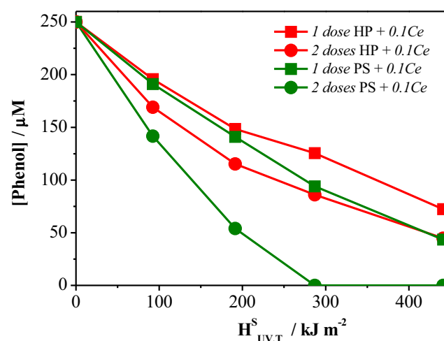
Fig. 6 Disappearance of phenol as a function of solar exposure in the presence of 0.1Ce and HP or PS. Reaction conditions: catalyst 0.1Ce = 1.0 \text{ g L}^{-1} , [\text{phenol}]_0 = 250 \mu\text{M} , PS or HP = 1 or 2 doses
