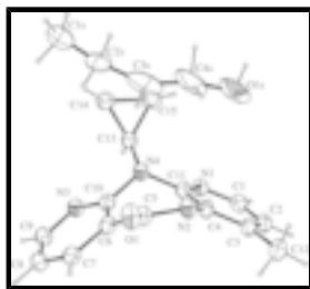
Fig. 1. The molecular structure of the butanol solvate of Nervirapine, showing the atom-labelling scheme. Displacement ellipsoids are drawn at the 30% probability level. H atoms are represented as small spheres of arbitrary radius.
