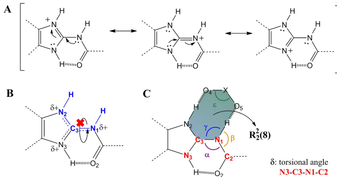
Scheme 3 (A) Detail of resonance structures of mebedazolium cation (MBZH + ). (B) Conformation around the partial double bond C 3 -N 1 in heterosynthon I. (C) Representative conformational parameters in heterosynthon I.
