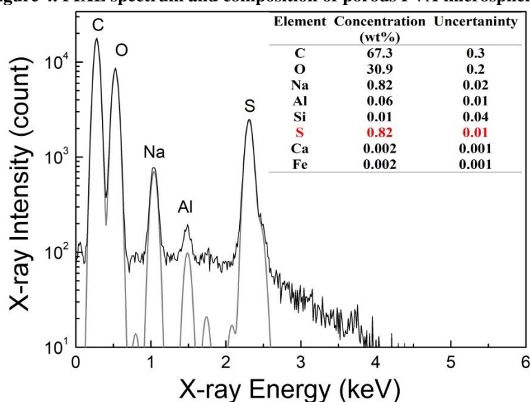
Figure 4. PIXE spectrum and composition of porous PVA microspheres.
