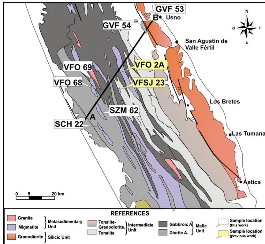
Fig. 2. Simplified geologic map of study area, from the inset of Fig. 1b. Sample locations for this study are shown, along a transverse across the entire range from the deepest to the shallower level. Paleo-up is to the northeast. Simplified geologic map modified from Mirrè (1976), Otamendi et al. (2009) and Vujovich et al. (1996).
