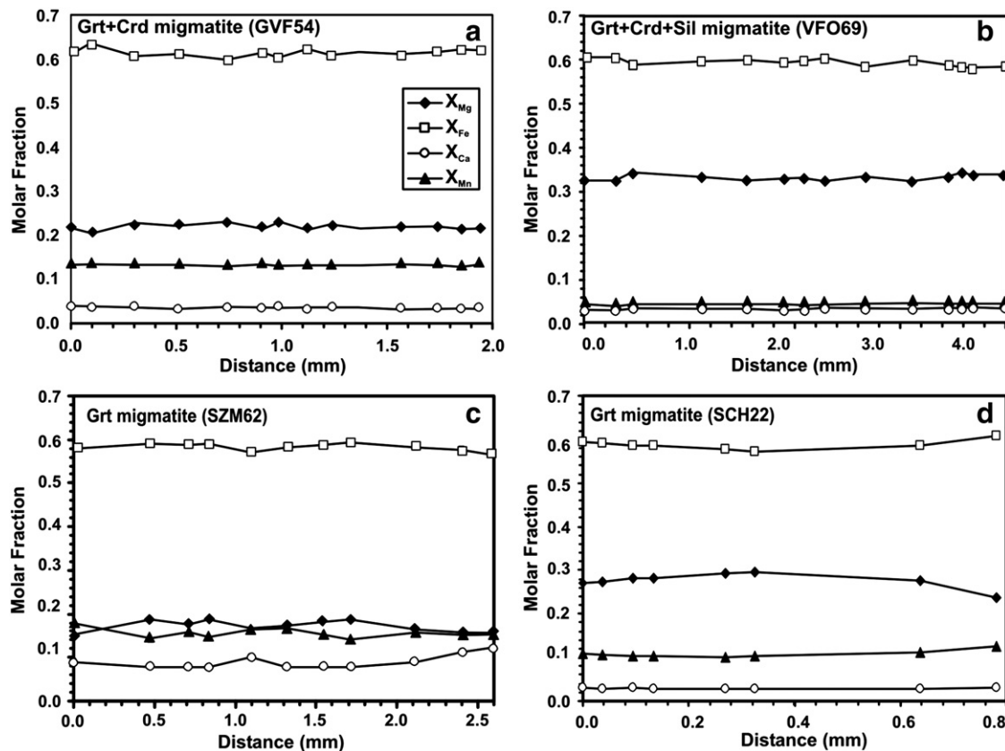
Fig. 4. Chemical profile for garnet porphyroblasts from the different migmatites types recognized in the central part of the Valle Fértel section.
