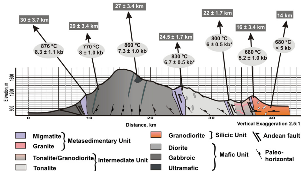
Fig. 7. Cross-section through the central part of the Sierra of Valle Fértil showing P–T conditions and estimated depths. *Data taken from Otamendi et al. (2008) and Tibaldi et al. (2011).
