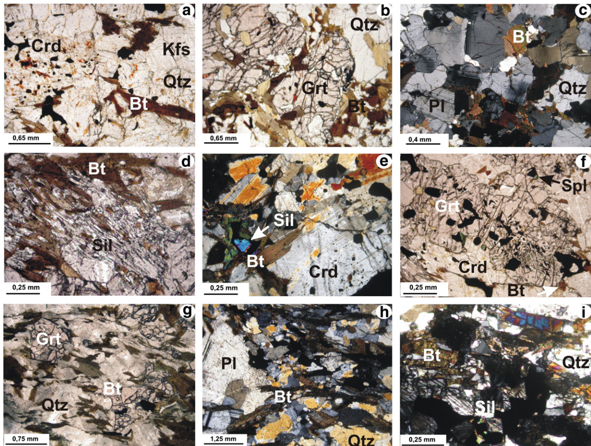
Fig. 3. Photomicrographs of the migmatites from the central part of the Sierra de Valle Fétil. (a) Typical granoblastic texture in cordierite-bearing migmatites (VFG53). (b) Mesocratic domain in garnet–cordierite-bearing migmatite (VFG54) showing the presence of small, euhedral garnet and garnet porphyroblast with poikilictic inclusions of biotite, oxides, and rounded quartz. (c) Leucosomes dominated by fine to medium-grained quartz and euhedral grains of plagioclase, showing equigranoblastic texture in garnet–cordierite-bearing migmatite (VFG54). (d) Coarse-grained aggregate of idioblastic sillimanite intergrown with quartz and biotite in garnet–cordierite–sillimanite-bearing migmatite (VFO68). (e) Clustered grains of idioblastic cordierite within the leucosome of migmatite VFO69. Cordierite also occurs as poikilictic porphyroblasts including several grains of biotite, sillimanite, and quartz. Cordierite is partly pinnitized and porphyroblasts commonly show polysynthetic twins. (f) Garnet porphyroblasts with reabsorbed rims that include biotite, quartz, and oxides (VFO68). (g) Typical granolepidoblastic texture in garnet-bearing migmatites, mesosomes consisting of biotite, sillimanite, garnet, quartz, plagioclase, and Fe–Ti oxides. (h) Foliation in garnet-bearing migmatite defined by mineral preferred orientations of biotite, plagioclase, elongated quartz, and prismatic sillimanite. (i) Idioblastic to subidioblastic sillimanite intergrown with quartz and biotite along the foliation planes. Mineral abbreviations after Kretz (1983).
