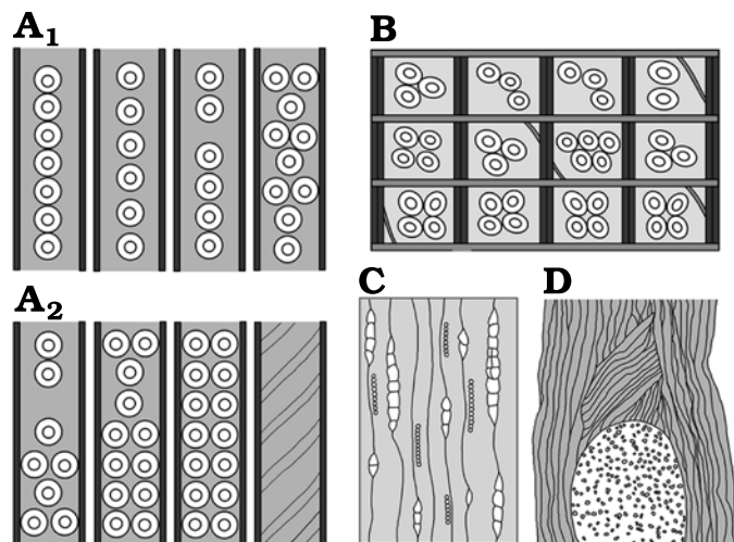
Fig. 4. Schemes showing anatomical characters of Baieroxylon cicatricum . A. Tracheid radial pitting patterns ( A_1 , A_2 ). B. Cross field pitting. C. Radial system. D. Detail of scar.
