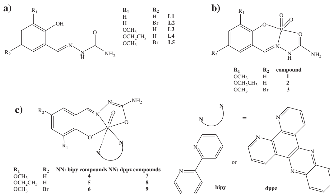
Fig. 1. a) Salicylaldehyde semicarbazone derivatives L selected as ligands (L1–L5); b) new [V^{VO}_2(L-H)] complexes 1–3; c) new [V^{IV}O(L-2H)(NN)] complexes, where NN = bipy (4–6) or dppz (7–9).
