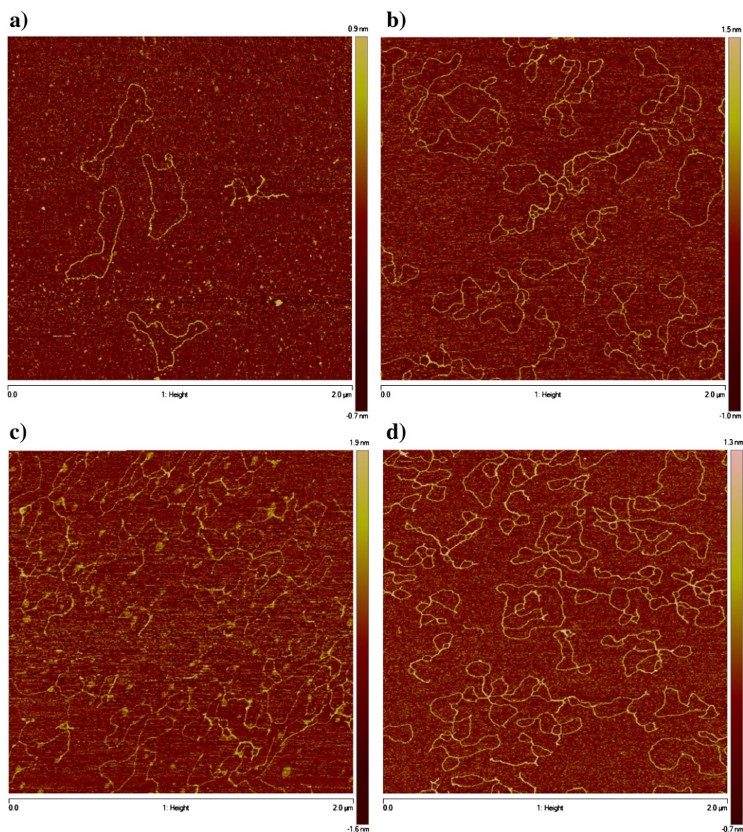
Fig. 6. AFM images showing the modifications suffered by pBR322 DNA due to the interaction with the dppz-containing V^{IV}O -compounds: a) pBR322 DNA b) 7 , [ V^{IV}O(L3-2H)(dppz) ], c) 8 , [ V^{IV}O(L4-2H)(dppz) ], d) 9 , [ V^{IV}O(L5-2H)(dppz) ] for molar ratio compound: DNA base pairs 1:5 and 24 h incubation at 37 °C.
