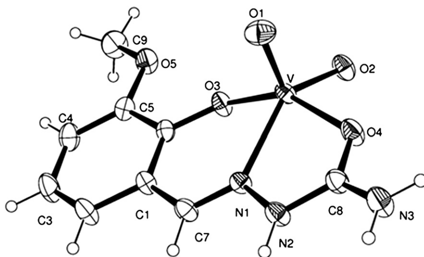
Fig. 2. ORTEP drawing depicting a view of [V IV O 2 (L3-H)] showing the labeling of the non-H atoms and their displacement ellipsoids at the 50% probability level.
