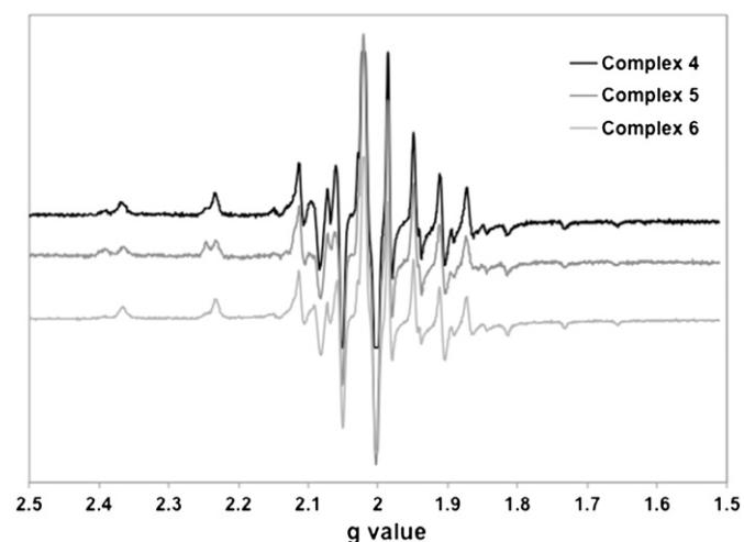
Fig. 3. 1st derivative EPR spectra of frozen solutions (77 K) of [V IV O(L-2H)(bipy)] complexes, 4-6, after dissolution in DMF (ca. 3 mM).
