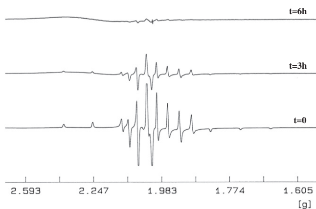
Fig. 4. Changes observed with time in the EPR spectra of a frozen solution (100 K) of complex [\text{V}^{\text{IV}}\text{O}(\text{L3-2H})(\text{dppz})] , 7 , after dissolution in DMF (ca. 3 mM).
