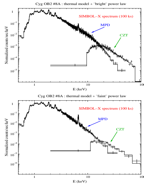
Fig. 2. Synthetic SIMBOL-X MPD and CZT spectra of Cyg OB2 #8A for two different assumptions on the flux of the power law.
