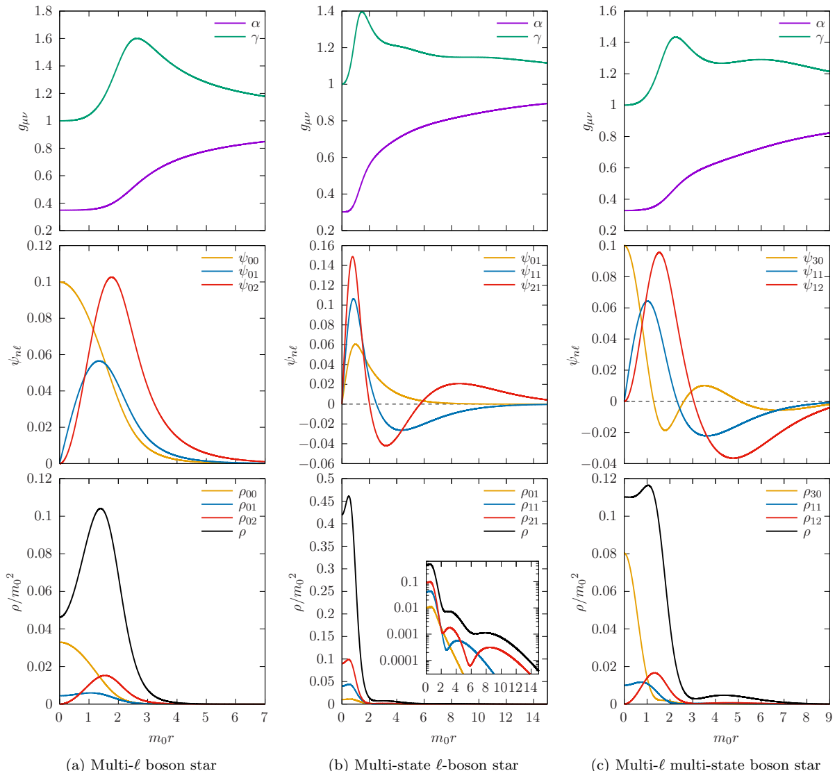
FIG. 1: As examples we describe here three particular solutions, each one of a different type, as indicated in the subfigures. For all cases we show the metric components, \alpha(r) and \gamma(r) (top panels); the state components \psi_{n\ell}(r) (middle panels); and the energy density \rho(r) , as well as the individual components \rho_{n\ell}(r) (bottom panels). Note that \rho can be obtained simply by summing its components (including all degenerate states in m ). Thus, we have \rho = \rho_{00} + 3\rho_{01} + 5\rho_{02} in (a), \rho = 3\rho_{01} + 3\rho_{11} + 3\rho_{21} in (b), and \rho = \rho_{30} + 3\rho_{11} + 5\rho_{12} in (c). We show more properties of these solutions in Table III. Finally, we note that the actual numerical integration domain in r is much larger than what is shown (for clarity) in the figures.
