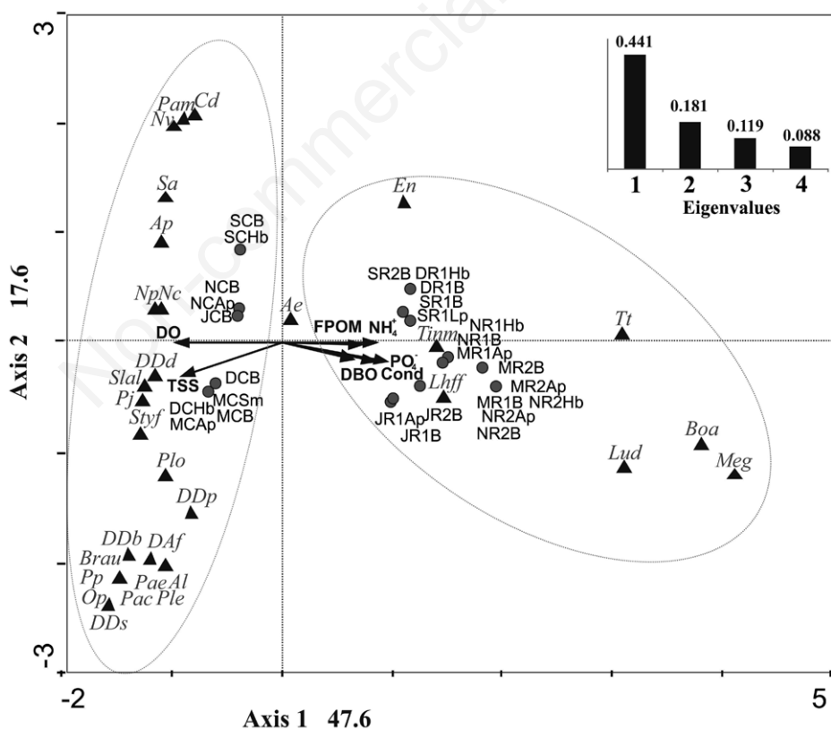
Fig. 2. Canonical-correspondence-analysis ordination of oligochaete species according to the physicochemical parameters at the study sites. Triangles, species ( cf. abbreviations in Tab. 2); gray circles, sites. Sampling dates: N, November; M, March; J, June; S, September; D, December. C, Carnaval site; R1, Rodríguez Site 1; R2, Rodríguez Site 2. B, benthos; Hb, H. bonariensis ; Sm, S. montevidensis ; Ap, A. philoxeroides ; Lp, L. peploides . Physicochemical parameters: fine particulate organic matter, FPOM; dissolved oxygen, DO; conductivity, Con; phosphate, P-PO_4^{3-} ; ammonium, N-NH_4^+ ; total suspended solids, TSS. The inset gives the eigenvalues for the four axes.
