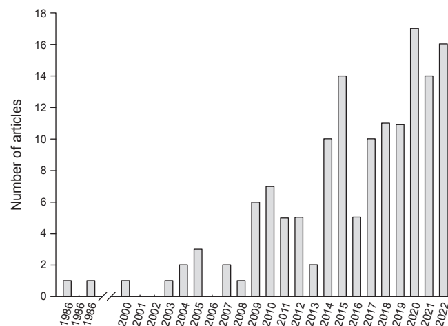
Fig. 2. Frequency of published articles on seabird behavioral flexibility between 1986 and 2022. No articles were published between 1989 and 1999.
