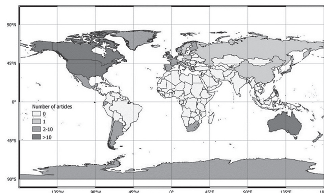
Fig. 3. Geographical distribution of the seabird behavioral flexibility studies analyzed in this review
