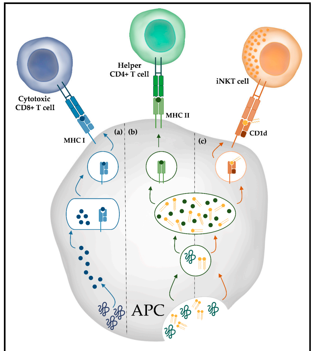
Figure 2. Cytotoxic cellular responses are induced after protein and glycan presentation on antigen-presenting cells. To induce an effective cytotoxic response directed at tumour cells, antigen-presenting cells process and present antigens to T and/or invariant natural killer T (iNKT) cells. T cell-dependent or thymus-dependent antigens are processed and presented on (a) major histocompatibility complex class I (MHC I) or (b) class II (MHC II) molecules to CD8+ or CD4+ T cells, respectively, depending on whether they are endogenous or extracellular proteins. CD8+ T cells will mediate the lysis of tumour or pathogen-infected cells, while the CD4+ T cell subpopulation will induce B cell differentiation into memory or antibody-secreting plasma cells, enabling the generation of antibodies and eventually a long-lasting immune response. (c) Conversely, gangliosides and glycolipids in general are presented via the CD1d receptor expressed by antigen-presenting cells. CD1d antigen presentation will further activate the iNKT cell subpopulation.
