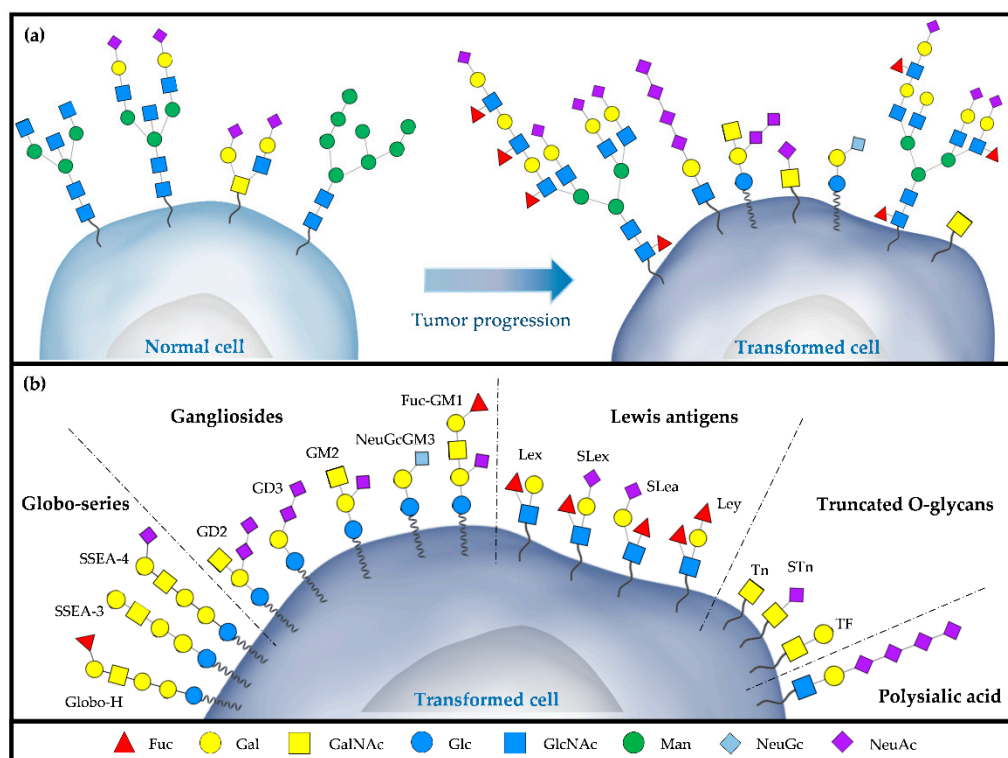
Figure 1. Schematic representation of the altered glycan expression that occurs during tumour progression. (a) Aberrant glycosylation in malignant transformation. Tumour cells show high expression of sialylated and fucosylated glycans, overexpress glycosphingolipids, and demonstrate increased expression of immature truncated O-glycans, which are almost absent in normal cells. (b) Tumour-associated carbohydrate antigens (TACAs) can be divided into five groups according to their structural similarities: (1) The globo-series family includes Globo-H, SSEA-3, and SSEA-4. (2) Gangliosides are glycosphingolipids with at least one sialic acid as a terminal glycan. The main family members are GD2, GD3, GM2, NeuGcGM3, and FucGM1. (3) Lewis antigen structures comprise terminal Lex, SLex, SLea, and Ley. (4) Truncated O-glycans include Tn, STn, and TF antigens. (5) Polysialic acid glycans are also expressed in tumour cells.
