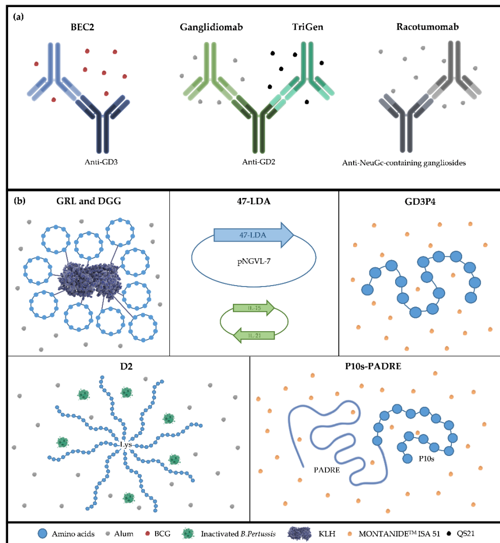
Figure 3. Schematic representation of the active immunotherapies directed at TACAs that have reached preclinical or clinical stages so far. (a) Therapeutic approaches based on anti-idiotypic (Id) antibodies. Ab1, which recognises GD3, GD2, and NeuGc-containing glycoconjugates was used to develop BEC2, ganglidiomab, TriGem, and racotumomab anti-Id antibodies. When administered in patients formulated with their specific adjuvants, all of these anti-Id antibodies demonstrated the induction of specific Ab3 able to recognize the nominal TACA. (b) Mimetic peptide-based therapeutic strategies. GRL and DGG are circularised decamers that mimic GD2 ganglioside. Each decamer is conjugated to KLH and finally adjuvanted in aluminium hydroxide (alum). The administration of the DNA vaccine 47-LDA induces the synthesis of a GD2 mimetic peptide when combined with an additional plasmid containing IL-15 and IL-21 sequences as immunostimulators. The mimetic peptide GD3P4 resembles the GD3 ganglioside structure. When formulated in MONTANIDE™ ISA 51, is able to induce an anti-GD3 humoral response. Regarding immature truncated O-glycans, the so-called D2 strategy is based on 15-mer peptides in a single molecule, which are recognized by a TF-specific lectin. Its final formulation with alum and inactivated B. pertussis induces anti-TF antibodies. Finally, the mimetic peptide P10s conjugated with the pan-T cell carrier PADRE and MONTANIDE™ ISA 51 as an adjuvant induces an immune response mainly against GD2 and Ley when administered to patients. P10s-PADRE is the first mimetic peptide to reach clinical trials and show promising results since it also induces a cellular immune response.
