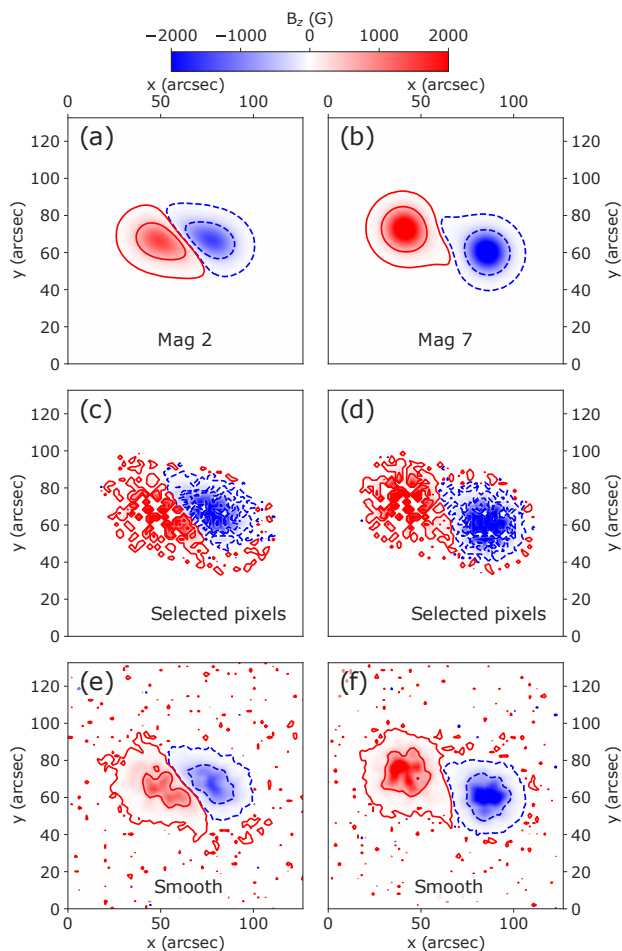
Fig. 6. Example of the model generator: (a)-(b) Magnetogram 2 and 7 of the seed model ( M_0 ). (c)-(d) Random selection of pixels for each magnetogram ( M_2 ). (e)-(f) Simulated data generated from panels (c) and (d), after applying a Gaussian-smooth filter and normal noise ( M_4 ). The color convention is the same as in Fig. 1.
