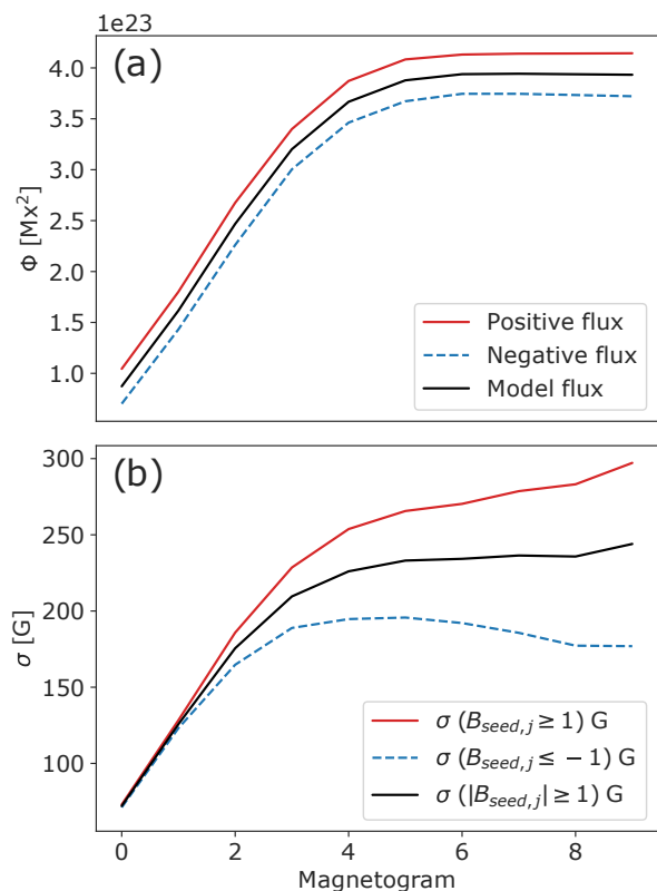
Fig. 8. Evolution of the LOS magnetic flux and the estimated \sigma for a single generated AR. (a) Evolution of magnetic flux for the generated AR shown in Fig. 6e,f. Solid-red and dashed-blue lines are the positive and negative flux, respectively. The black line shows the seed model magnetic flux. (b) Estimated \sigma using Eq. (5) applied to the seed model and the generated AR. The red-solid (blue-dashed) line corresponds to \sigma for the positive (negative) polarity. The black line corresponds to \sigma estimated with all the pixels within the generated AR field.
