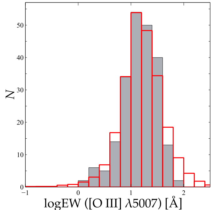
Figure 3. [O\text{ III}] \lambda 5007 rest-frame EW distribution of 220 GNIRS-DQS sources (solid gray histogram) and a similar distribution from Shen et al. (2011; red outline; scaled down by a factor of 500). See M21 for additional discussion. Forty sources did not meet our threshold of reliability for an [O\text{ III}] EW measurement that we require to be greater than 1 \text{ \AA} .
