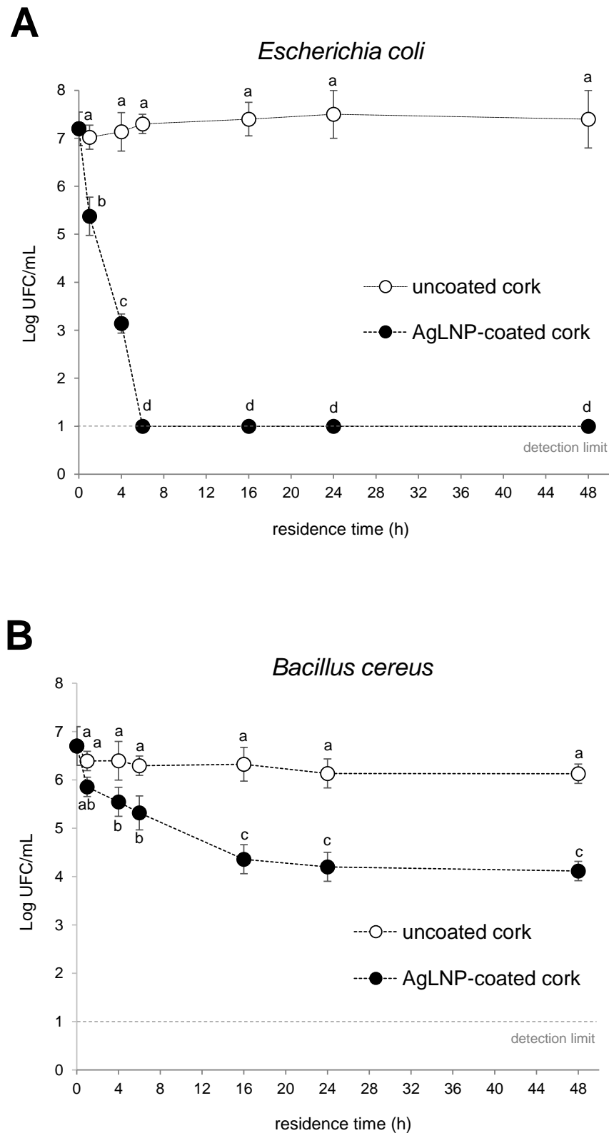
Figure 5. Antibacterial activity against E. coli (A) and B. cereus spores (B) of control uncoated- and AgLNP-coated cork acting as the filter medium in a point-of-use device for water disinfection. Different letters represent significant differences ( p < 0.05 ) between groups and at increasing residence time; e.g., “a” and “b” are statistically different from each other but not from “ab”. Data are reported as the mean value \pm standard error (S.E.) from three biological replicates ( n = 3 ) derived from independent experiments.
