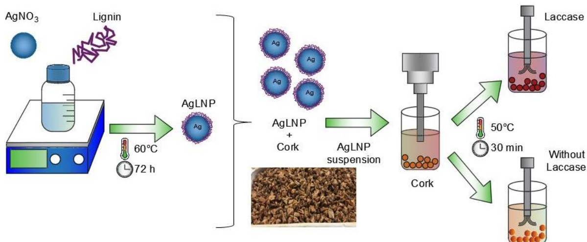
Figure 1. Synthesis and embedding of AgLNP in cork by the sonochemical technique.
