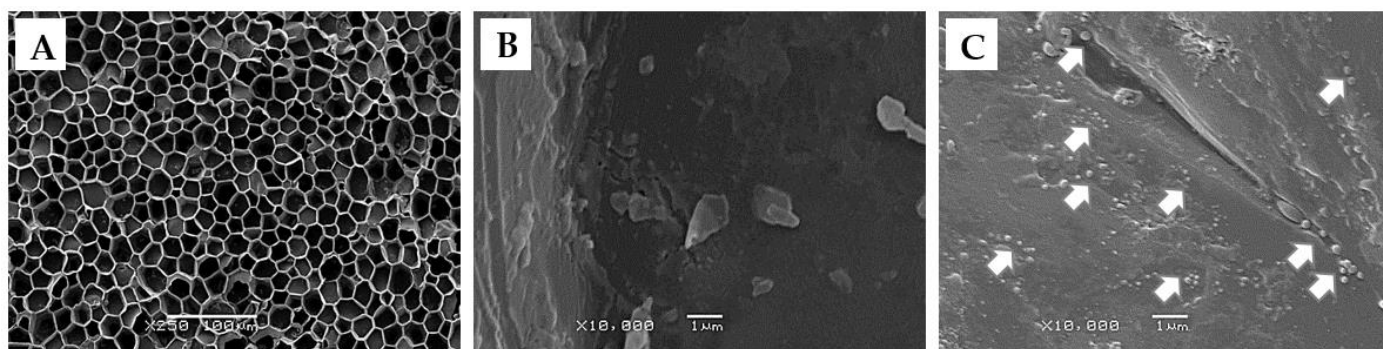
Figure 3. SEM microphotographs showing the ultrastructure of unmodified cork at two magnifications (A) = \times 250 and (B) = \times 10,000 ), and the ultrastructure of the AgLNP coated-cork (C). Note the presence of circular nanoparticles attached to the surface of the cork composite material in C (white arrows).
