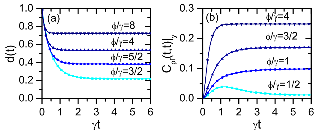
Figure 1. (a) Decay of the trace distance d(t) (Equation (38)) corresponding to the model (30). (b) Time dependence of the CPF correlation C_{pf}(t, t)|_y in the deterministic scheme [56] corresponding to the same model. The value of the quotient \phi/\gamma is indicated in each plot.
