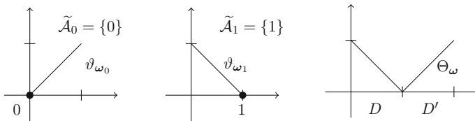
Fig. 3 Convex piecewise affine functions for other subsets
