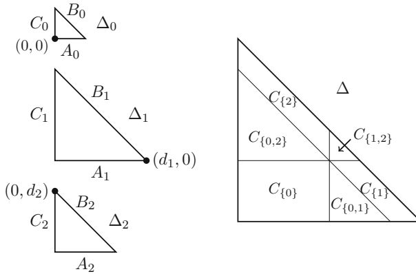
Fig. 4 A mixed subdivision in dimension 2
