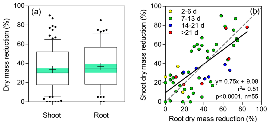
Fig. 4 Effect of waterlogging on shoot ( n=97 ) and root ( n=55 ) dry mass reductions (as % of controls) (a) and the relationship between shoot and root dry mass reductions (b, n=55 ). Boxes are 50% of the observations with the median shown as the horizontal line within each box, mean as ‘+’ within each box, and bars extending from each box are 10 and 90 percentiles; outliers are shown as ●. Data are from plants in pots ( n=12 ), hydroponic culture ( n=1 ) and field conditions ( n=9 ) reported in 22 peer-reviewed articles (data values, key experimental conditions, and references are given in Supplementary Table S2). Waterlogging (days) for experiments with
