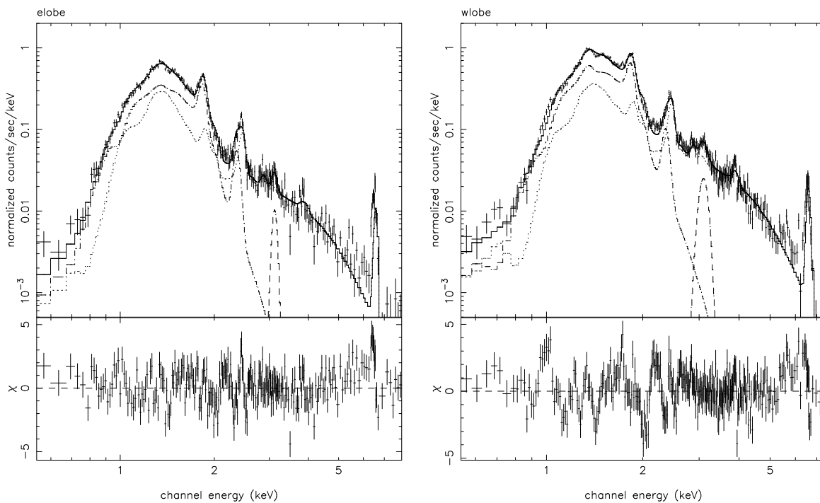
Fig. 11.— The data (crosses) and the fitted model for the eastern (left) and western (right) lobes of 3C 397. The model used is a two-component vshock model. A Gaussian line has been added to account for the line emission from Argon. The components of the model are shown as dashed lines. The bottom panel displays the residuals in units of sigmas. The parameters of the fits are summarized in Table 3. Both plots are shown on the same y-scale.
