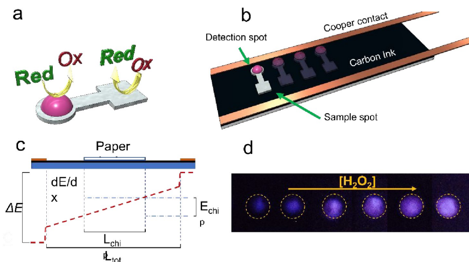
Figure 1. Schematic representation of the sensor including the principles of SEES. a) Scheme of the paper device indicating the reactions occurring in each spot, b) General overview of the SEES-ECL proposed method, c) Diagram showing electrical potential along the electrode, d) real captures of the ECL response using the smartphone. Conditions: 25 V, sample volume: 2.5 \mu\text{L} , [\text{H}_2\text{O}_2] 0.05 - 150 mM.
