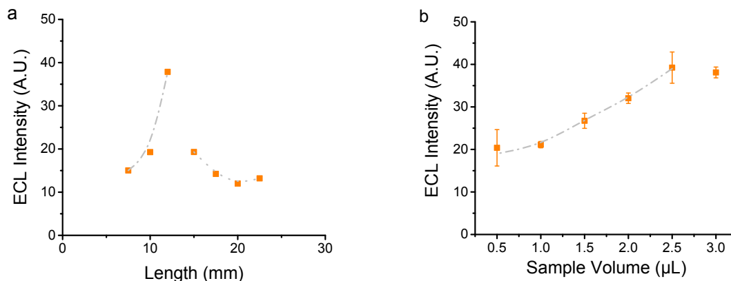
Figure 4a: ECL intensity as a function of the length of the paper device. Conditions: carbon paint electrode, E_{\text{tot}} = 25 V, sample volume = 2.5 \mu\text{L} , [\text{H}_2\text{O}_2] = 150 mM, read-out time = 23 sec.
