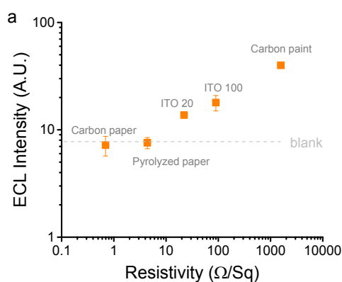
Figure 3a: Effect of the material selected for the electrode on the ECL response. Conditions: E_{\text{tot}} = 25 \text{ V} , sample volume = 2.5 \mu\text{L} , [\text{H}_2\text{O}_2] = 150 \text{ mM} , read-out time = 23 sec, device length = 12 mm.
