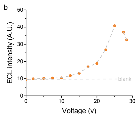
Figure 3b: Effect of the potential applied to the carbon paint electrode on the ECL response. Conditions: sample volume = 2.5 \mu\text{L} , [\text{H}_2\text{O}_2] = 150 \text{ mM} , read-out time = 23 sec, device length = 12 mm.
