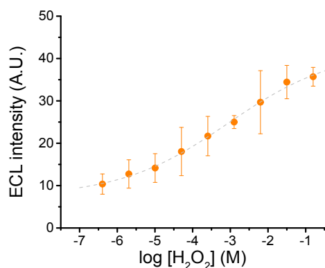
Figure 5. Calibration curve for Hydrogen peroxide as a function of ECL intensity. Conditions: carbon paint electrode, E_{tot} = 25 V, sample volume = 2.5 \mu L, read-out time = 23 sec, device length = 12 mm.
