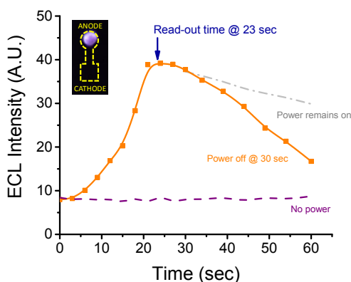
Figure 2. ECL intensity as a function of time, comparing the response of the device when no power was applied (control), when power was applied for only 30 sec, or when power was applied for 60 sec. The insert shows a picture showing the position of the detection spot with respect to the paper device. Conditions: E_{tot} = 25 V, sample volume = 2.5 \mu L, [H_2O_2] = 150 mM, device length = 12 mm.
